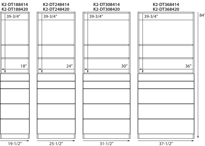
Drawer Floor Tower Frames with Small & Large Drawers & Adjustable Shelves 84" High, 14" or 20" Deep
