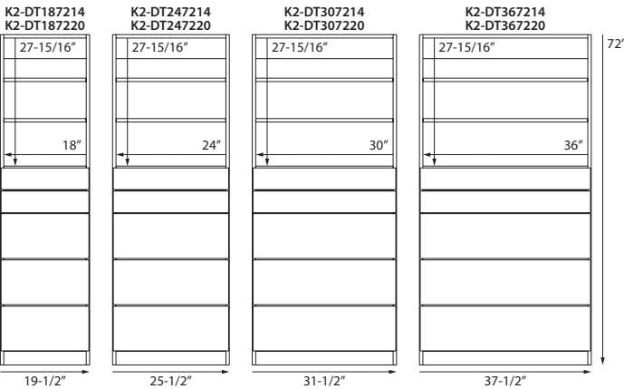
Drawer Floor Tower Frames with Small & Large Drawers & Adjustable Shelves 72" High, 14" or 20" Deep
