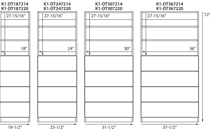
Drawer Floor Tower Frames with Large Drawers & Adjustable Shelves 72" High, 14" or 20" Deep
