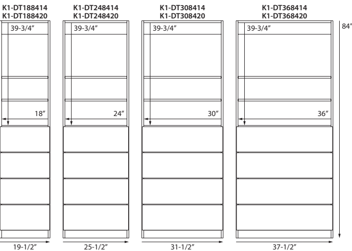
Drawer Floor Tower Frames with Large Drawers & Adjustable Shelves 84" High, 14" or 20" Deep
